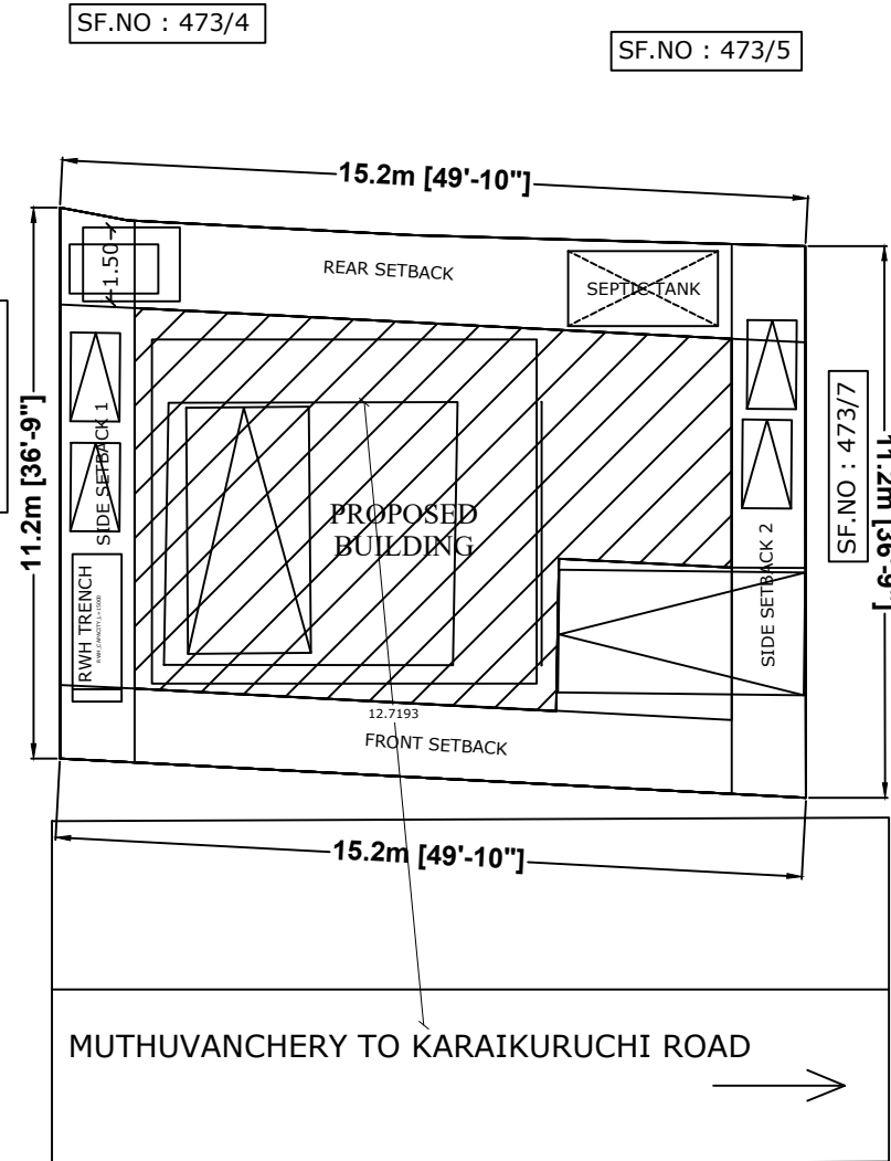
SITE PLAN
