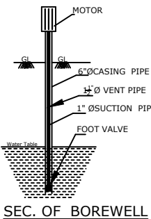
SEC. OF BOREWELL
