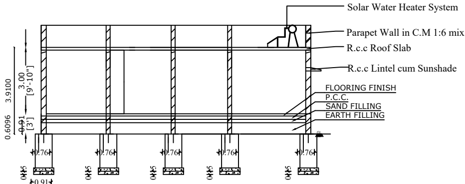
SECTION ON XX
