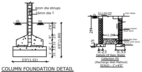
COLUMN FOUNDATION DETAIL
