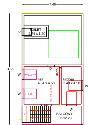
PROPOSED SECOND FLOOR & TERRACE FLOOR
