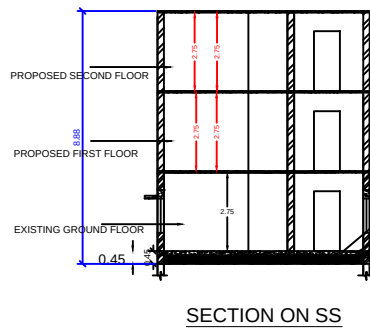
SECTION ON SS
