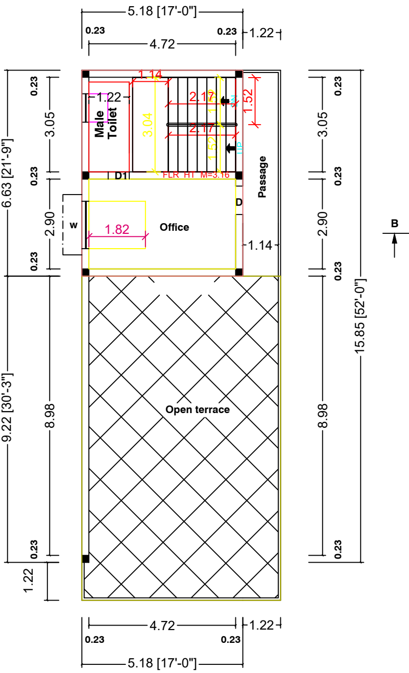
FLOOR-1 (FIRST) PLAN ( FACING EAST )
