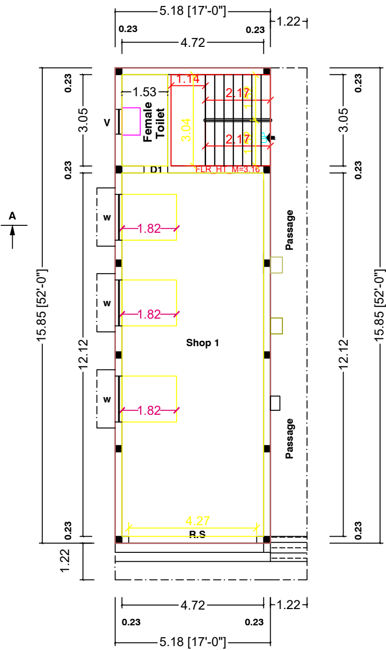
FLOOR-0 (GROUND) PLAN ( FACING EAST )
