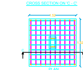
COLOUMN FOUNDATION DETAILS
