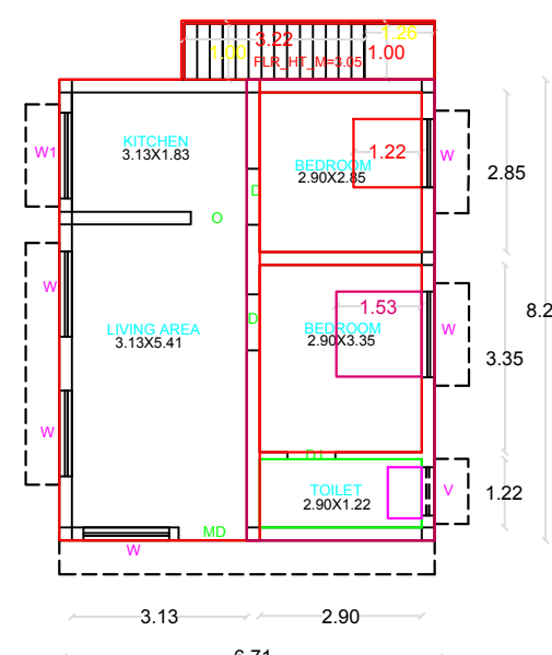
EX&PRO.GROUND FLOOR PLAN
