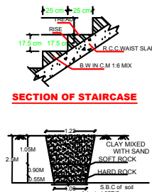
TRIAL PIT DETAILS
