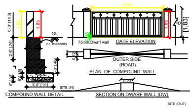
DETAILS OF COMPOUND WALL
