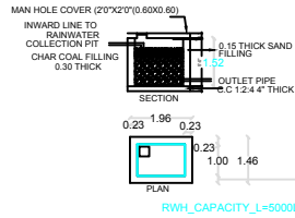
DETAILS OF RAINWATER HARVESTING
