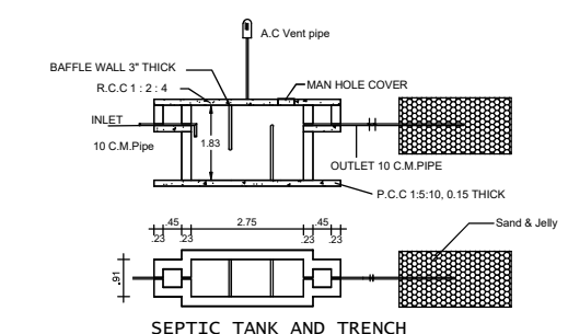
SEPTIC TANK AND TRENCH
