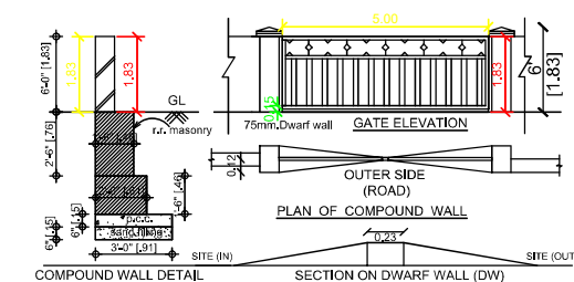
COMPOUND WALL DETAIL
