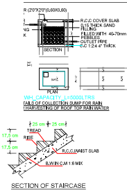
SECTION OF STAIRCASE
