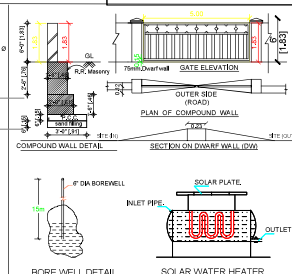
BORE WELL DETAIL SOLAR WATER HEATER
