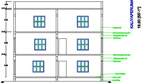
CROSS SECTION ON 'AB'
