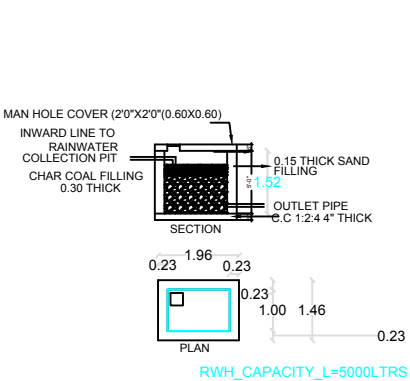
DETAILS OF RAINWATER HARVESTING
