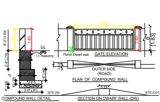
DETAILS OF COMPOUND WALL
