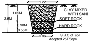
TRIAL PIT DETAILS
