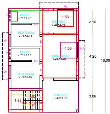
GROUND FLOOR AREA
