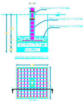
COLOUMN FOUNDATION DETAILS
