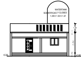
FRONT ELEVATION NORTH FACING.
