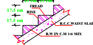
SECTION OF STAIRCASE
