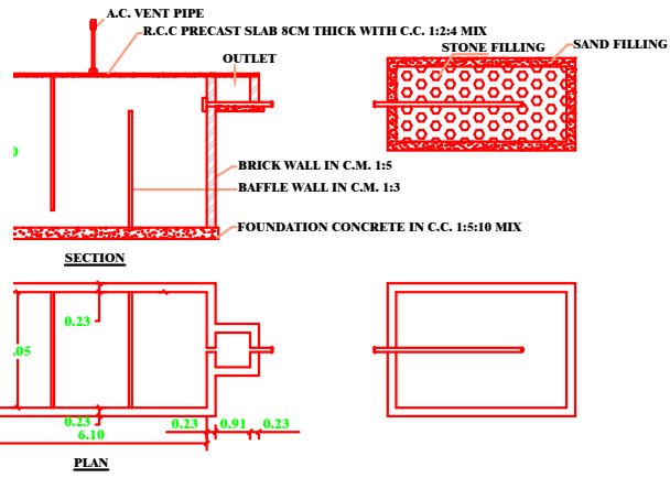
PLAN & SECTION OF SEPTIC TANK & DISPERSION TRENCH
