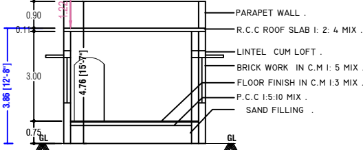
CROSS SECTION ON 'AB'
