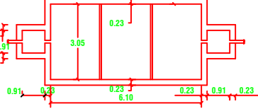
PLAN & SECTION OF SEPTIC TANK & DISPERSION TRENCH
