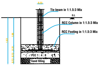
CROSS SECTION ON 'C - C'
