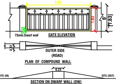
SECTION ON DWARF WALL (DW)
