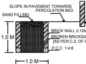
SECTION OF RAIN WATER PERCOLATION BED
