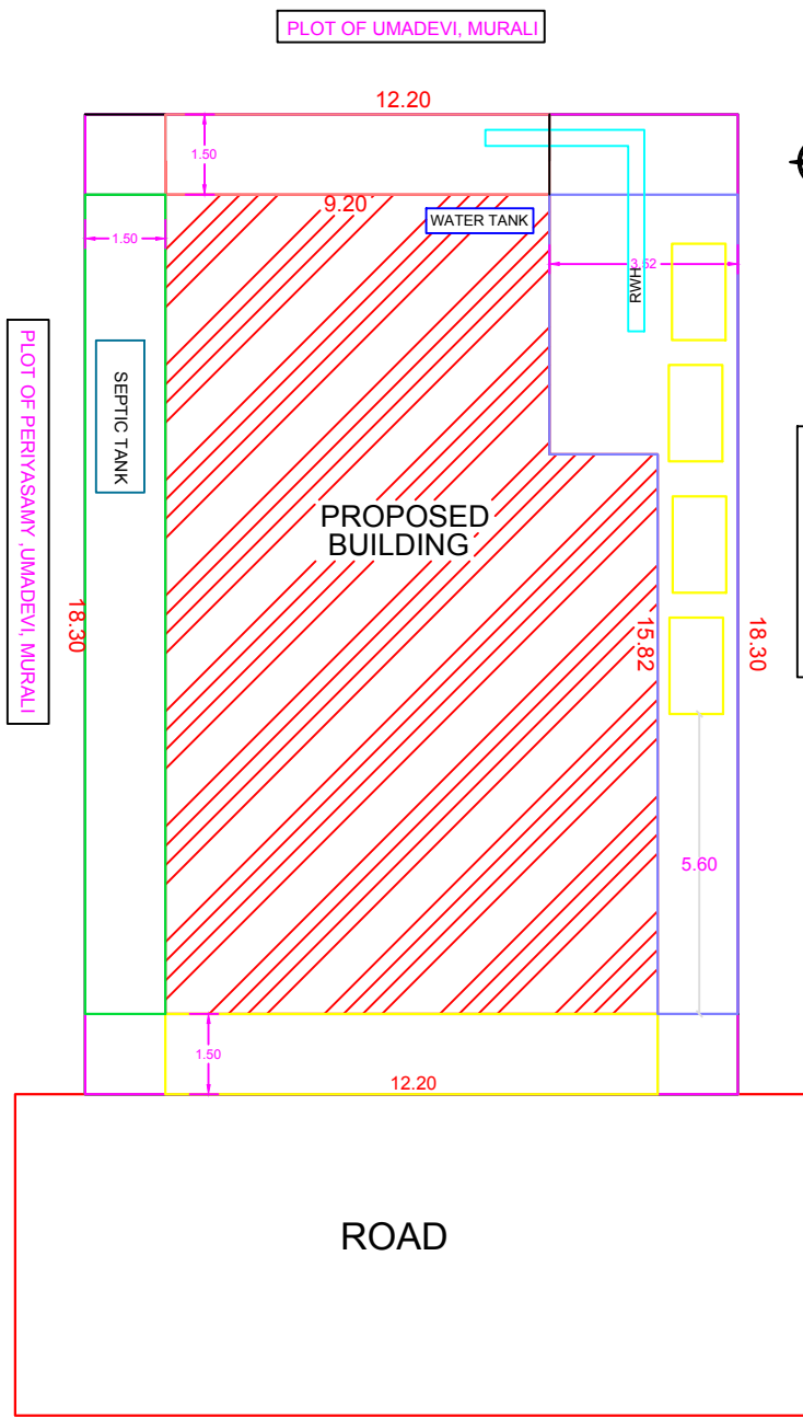
SITE PLAN
