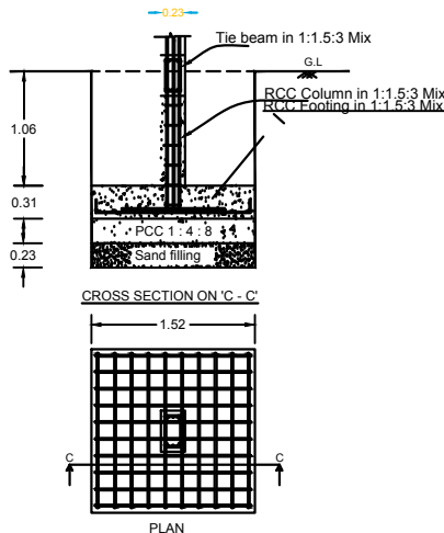
COLOUMN FOUNDATION
