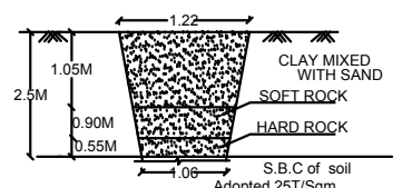
TRIAL PIT DETAILS
