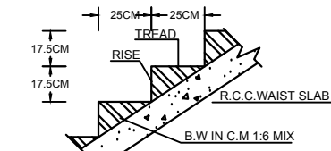
SECTION OF STAIRCASE
