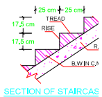
SECTION OF STAIRCASE
