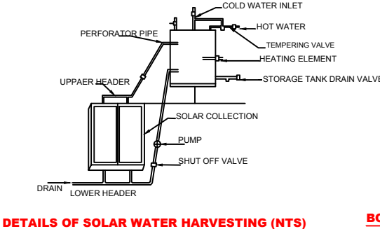
DETAILS OF SOLAR WATER HARVESTING (NTS)
