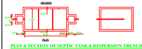
PLAN & SECTION OF SEPTIC TANK & DISPERSION TRENCH
