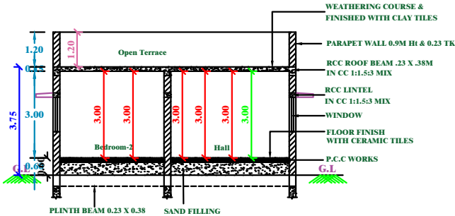
SECTION-XX
