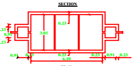
PLAN & SECTION OF SEPTIC TANK & DISPERSION TRENCH
