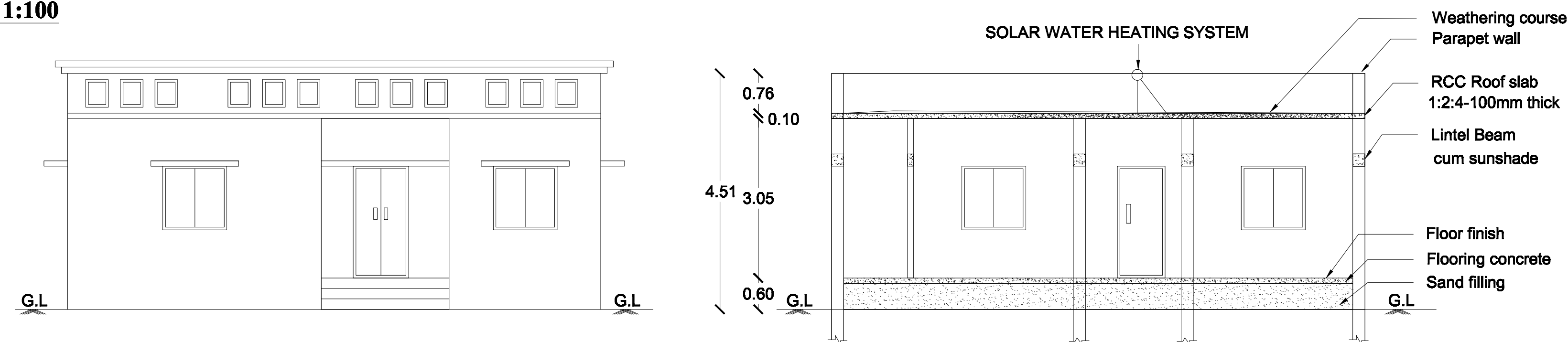
FRONT ELEVATION
