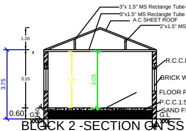
BLOCK 2 -SECTION ON SS
