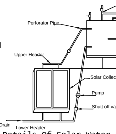
Details of solar water heater (NTS)
