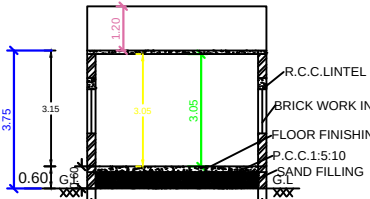
BLOCK 1 -SECTION ON SS
