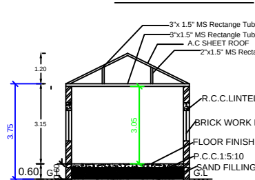
BLOCK 4 -SECTION ON SS
