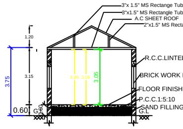
BLOCK 3 -SECTION ON SS
