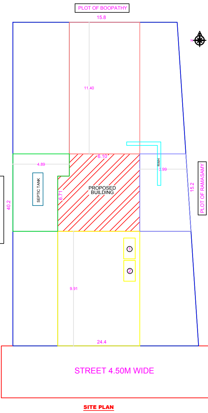
SITE PLAN
