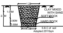
TRIAL PIT DETAILS
