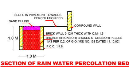
SECTION OF RAIN WATER PERCOLATION BED
