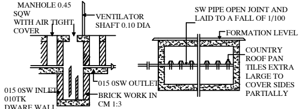
SECTION OF SEPTIC TANK
