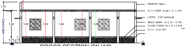
CROSS SECTION ON 'AB'
