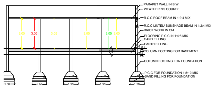
SECTION ON-AA
