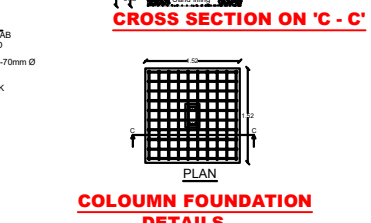
COLOUMN FOUNDATION DETAILS
