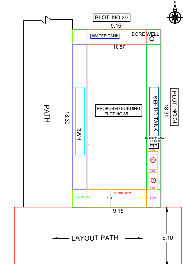
SITE PLAN
