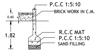
FOUNDATION DETAILS
