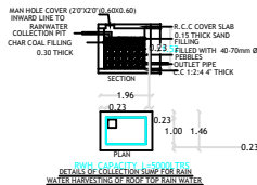
DETAILS OF COLLECTION PUMP FOR RAIN WATER (18" x 18" x 18")
