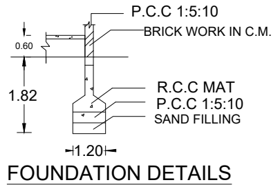
FOUNDATION DETAILS
