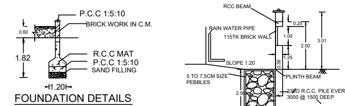
RAINWATER HARVESTING
