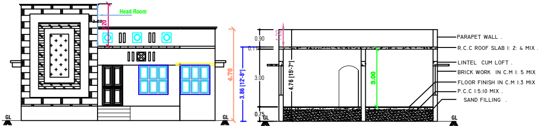
FRONT ELEVATION
