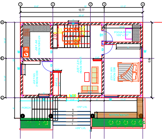
GROUND FLOOR PLAN (NORTH FACING)
