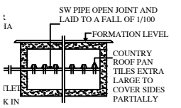
SECTION OF DISPERSION TRENCH
