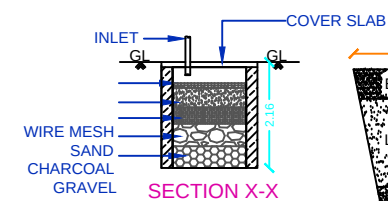
SECTION X-X
