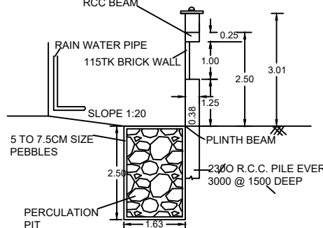
RAINWATER HARVESTING
