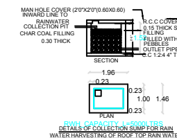
DETAILS OF RAINWATER HARVESTING
