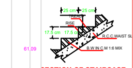
SECTION OF STAIRCASE
