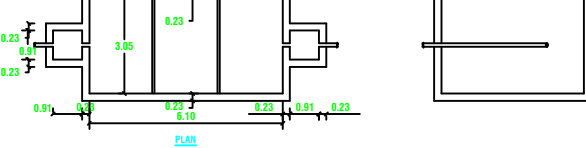
PLAN & SECTION OF SEPTIC TANK & DISPERSION TRENCH
