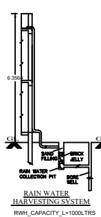
RAIN WATER HARVESTING SYSTEM
