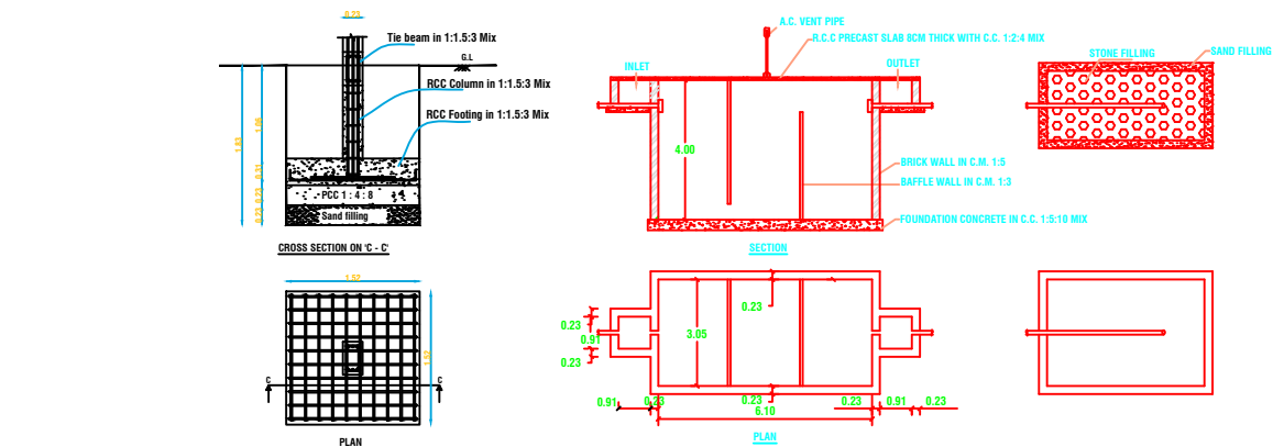
PLAN & SECTION OF SEPTIC TANK & DISPERSION TRENCH
