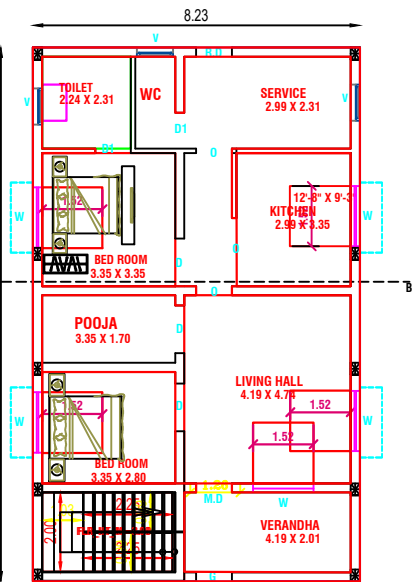
GROUND FLOOR PLAN (SOUTH FACING)
