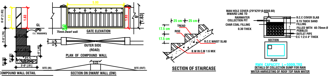
COMPOUND WALL DETAIL
