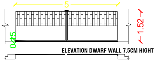
GATE ELEVATION
