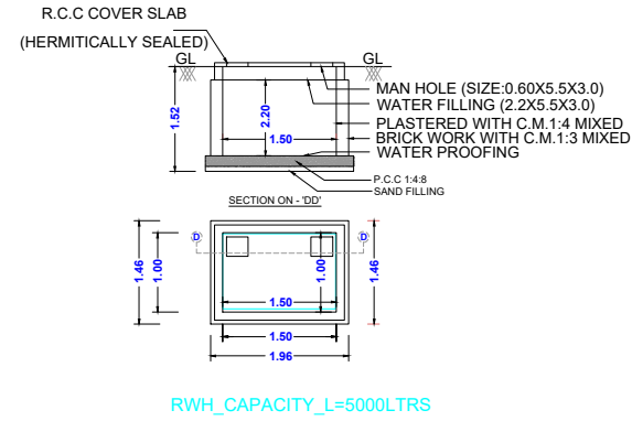
DETAILS OF COLLECTION SUMP FOR RAIN PLAN
