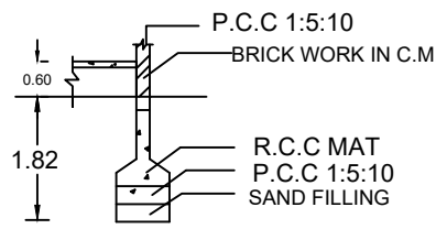
FOUNDATION DETAILS
