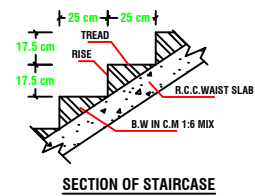
SECTION OF STAIRCASE
