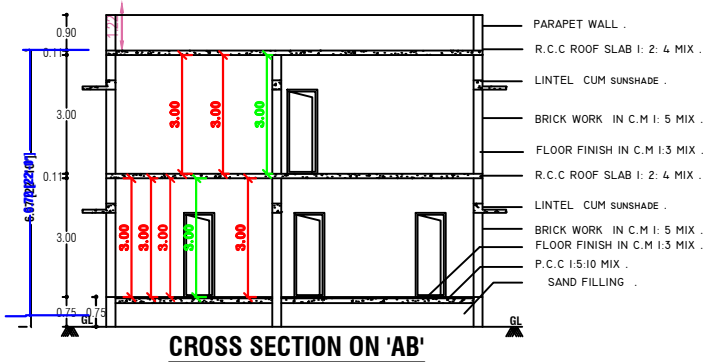
CROSS SECTION ON 'AB'
