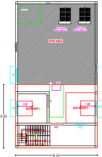
FIRST FLOOR PLAN PRO. FIRST FLOOR
