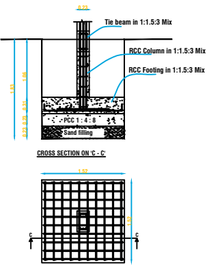
COLOUMN FOUNDATION DETAILS
