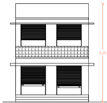
FRONT ELEVATION
