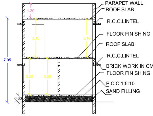
SECTION ON "SS "
