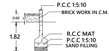
FOUNDATION DETAILS
