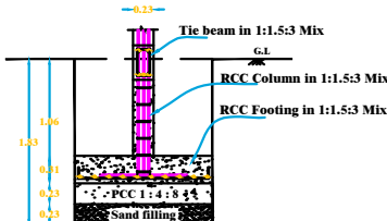
CROSS SECTION ON 'C - C'
