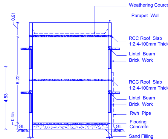
SECTION X-Y
