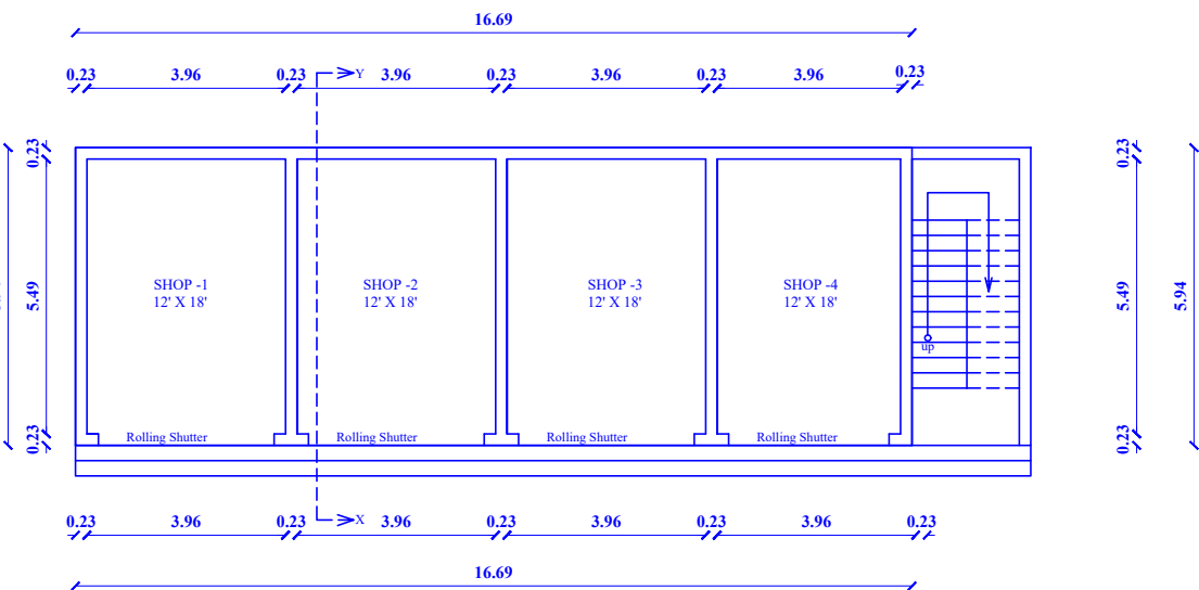
EXIG -GROUND FLOOR PLAN
