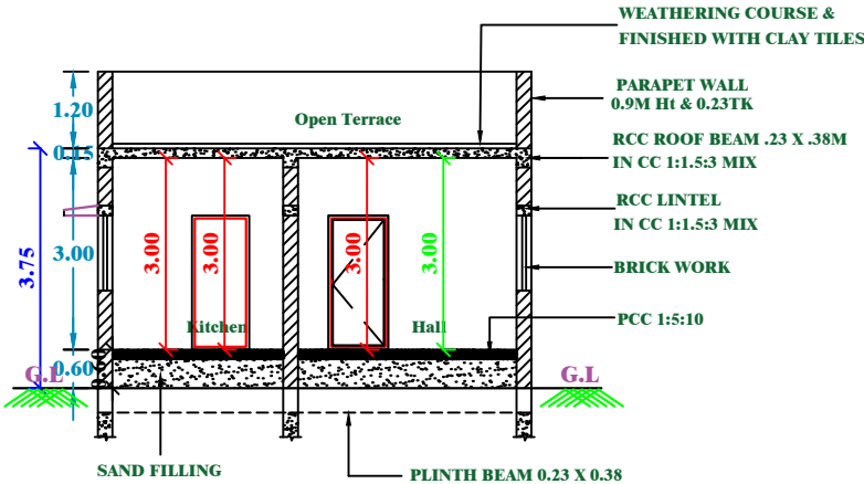
SECTION-XX
