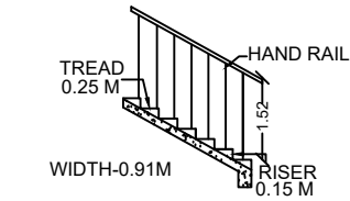
STAIRCASE DETAILS
