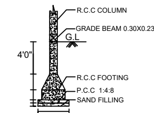
COLOUMN FOUNDATION DETAILS
