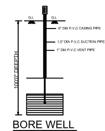
BORE WELL
