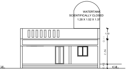
FRONT ELEVATION WEST FACING.
