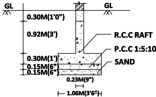
"FOUNDATION DETAILS"
