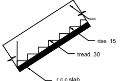
STAIR
