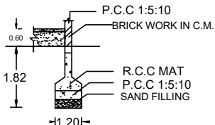
FOUNDATION DETAILS
