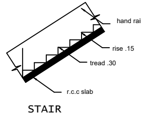
STAIR
